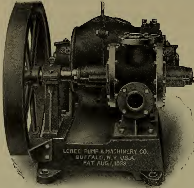
SPECIAL NO. 6 MOTOR PUMP For Pumping Lye, Soap, Oils, etc.
